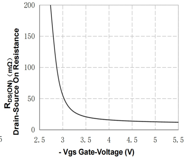
Figure 8. On-Resistance vs Gate Voltage
