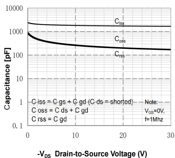
Figure 5. Capacitance Characteristics
